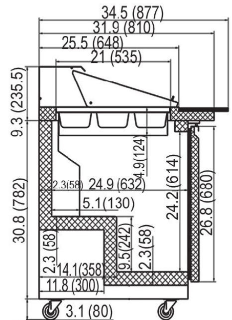
S72-MT-HC & S72-MT-SI-HC SIDE VIEW
