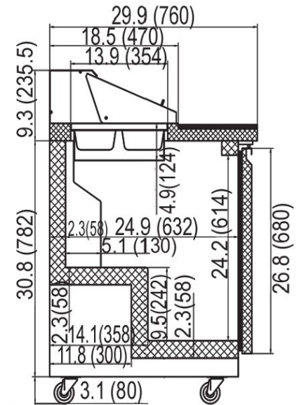
S72-MT-HC & S72-MT-SI-HC SIDE VIEW
