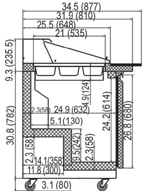
S61-MT-HC & S61-MT-SI-HC SIDE VIEW
