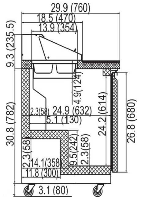
S61-HC & S61-SI-HC SIDE VIEW
