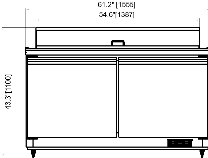
S61-HC & S61-SI-HC PAN VIEW
