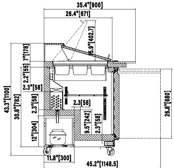
S36-MT-HC & S36-MT-SI-HC SIDE VIEW
