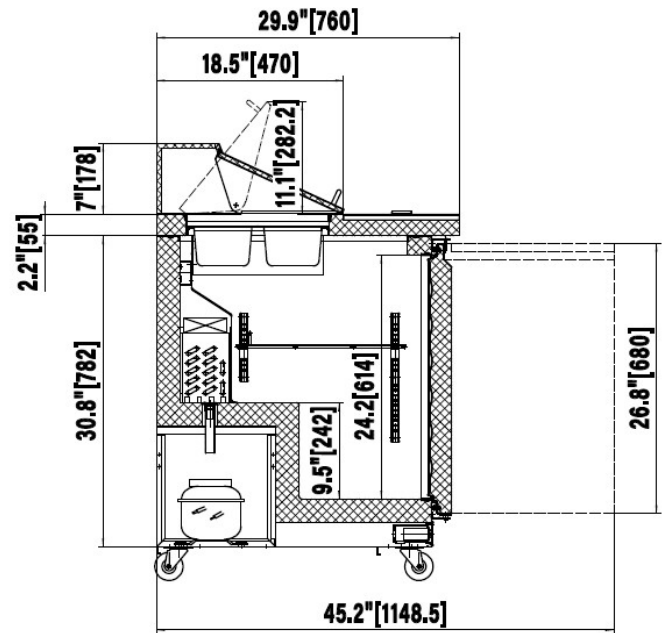
S36-MT-HC & S36-MT-SI-HC SIDE VIEW
