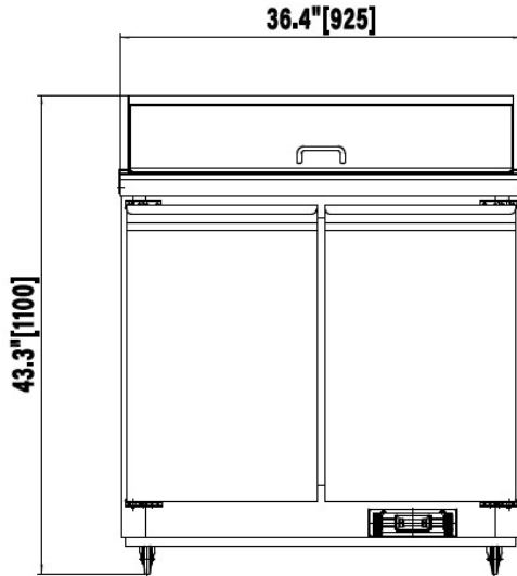
S36-HC, S36-SI-HC, S36-MT-HC, S36-MT-SI-HC FRONT VIEW
