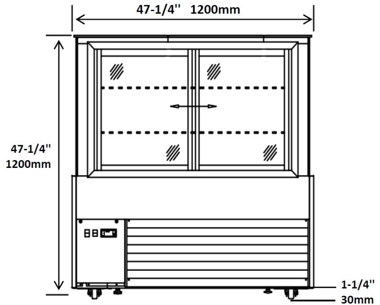
ECD47-2X REAR
