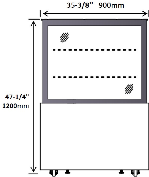
ECD47-2X FRONT
