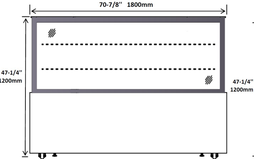
ECD71-2X FRONT
