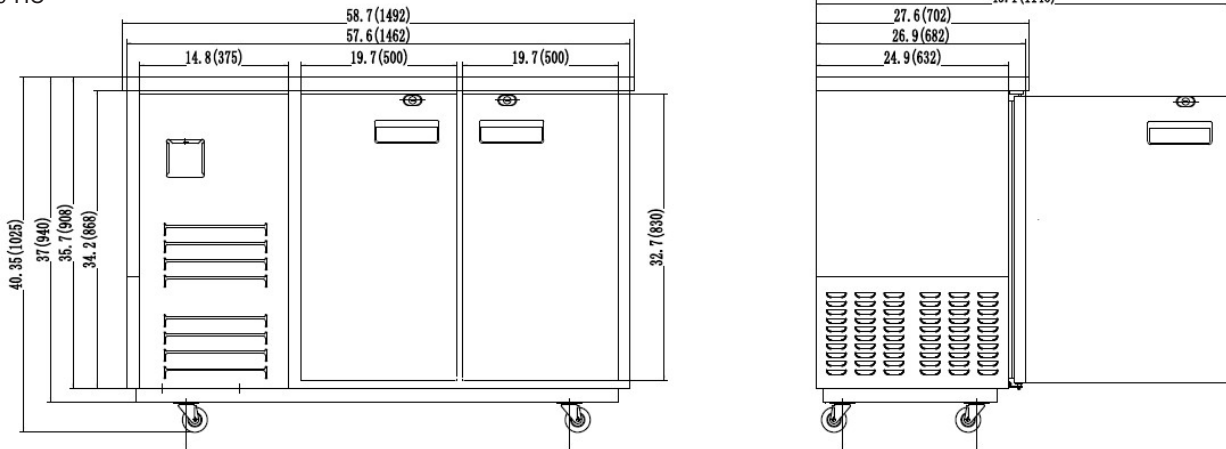
BB-2D-60-HC
