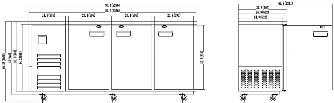
BB-3D-90-HC
