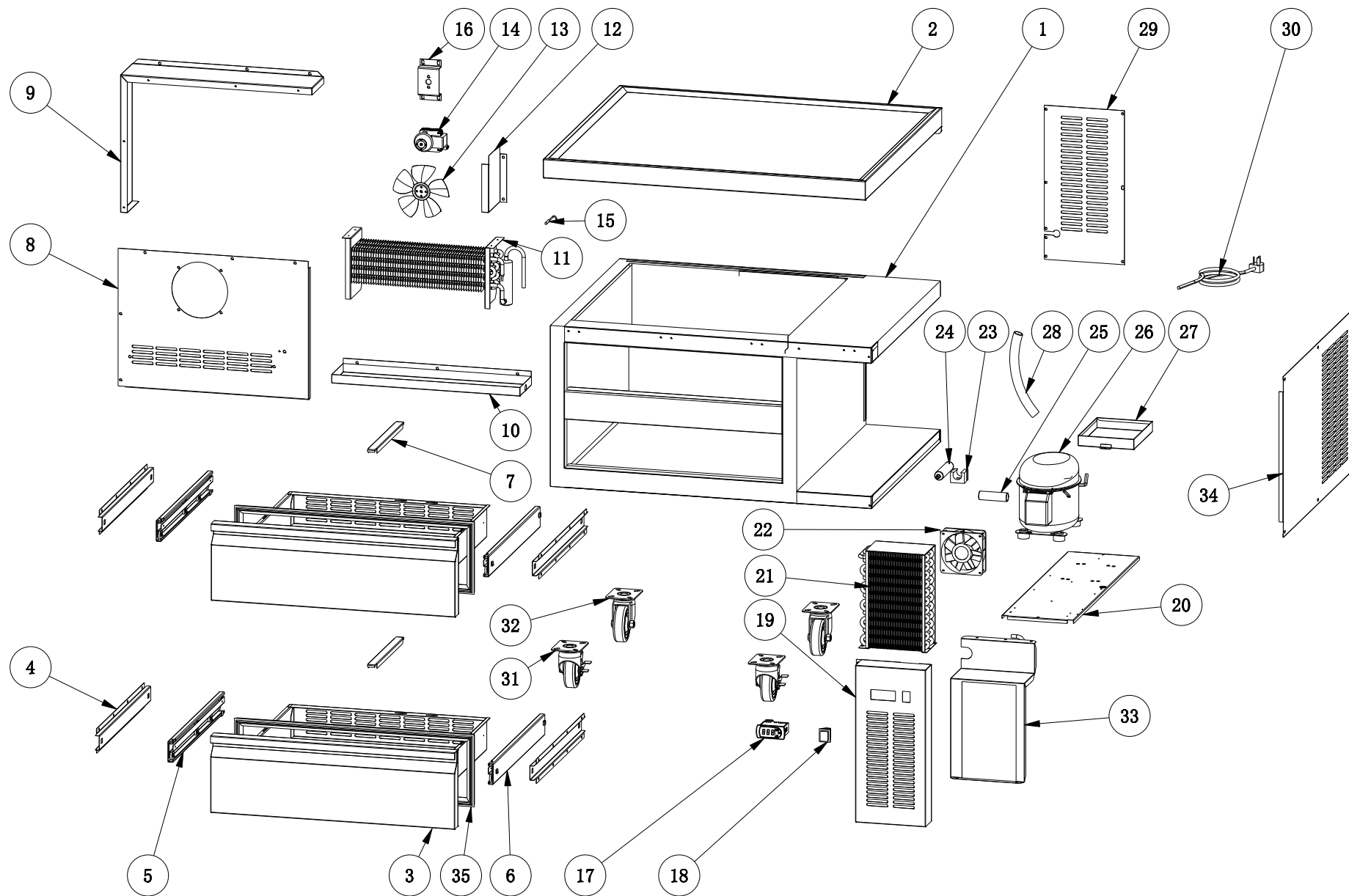
MODEL ECB48X
