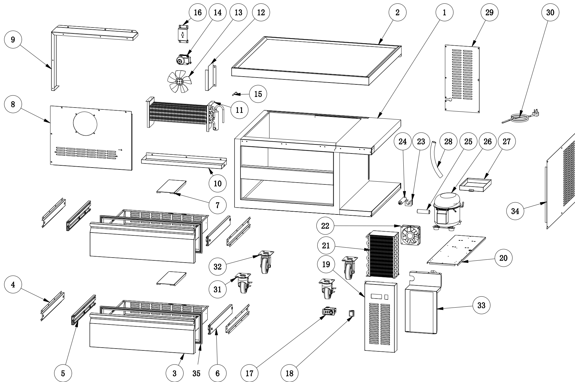
MODEL ECB36X
