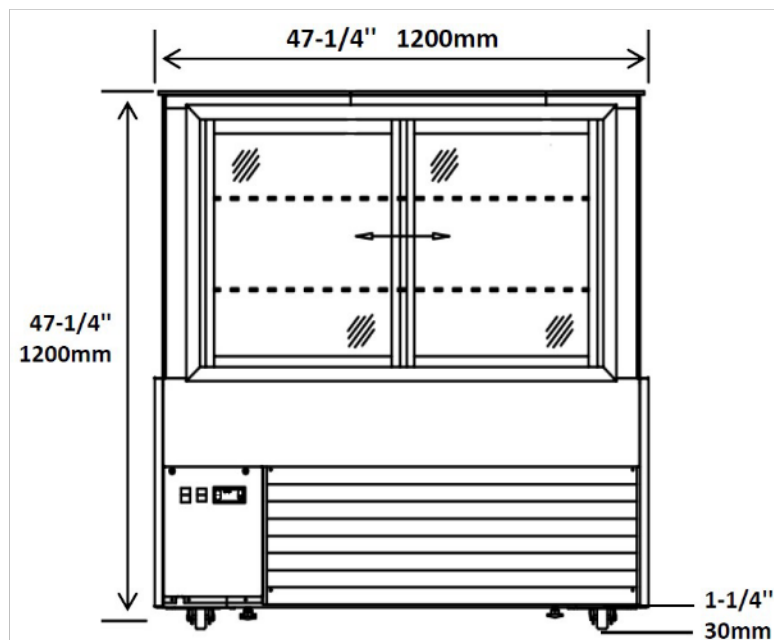
ECD47-2X REAR
