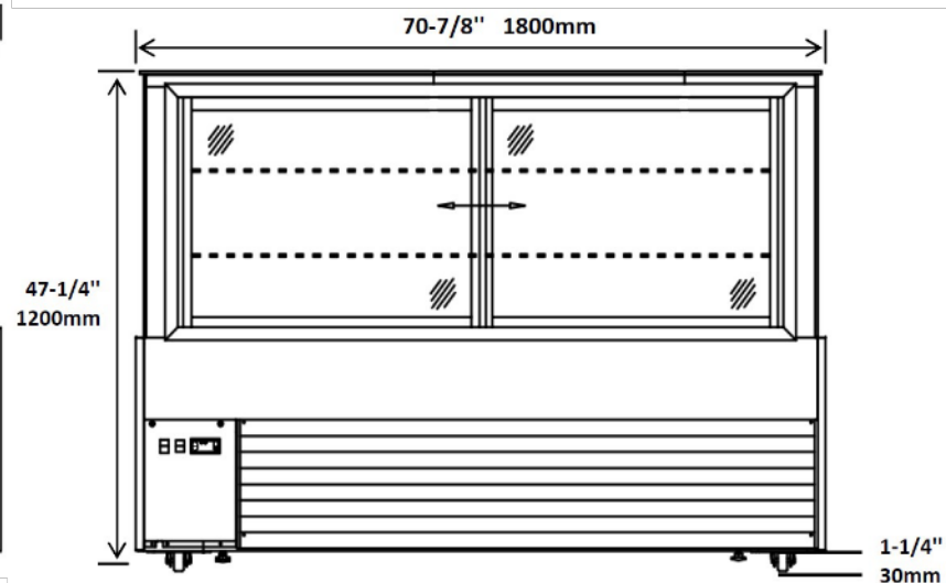
ECD71-2X REAR
