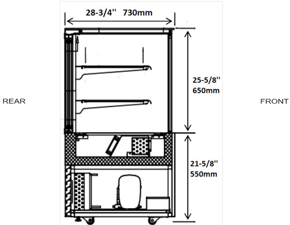
SIDE VIEW ALL
