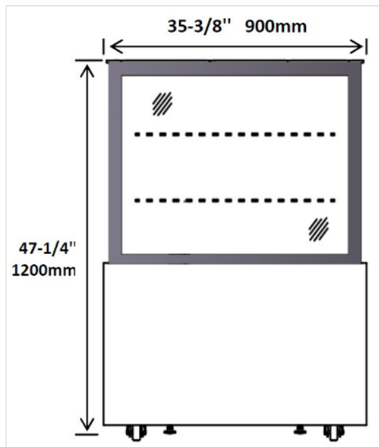
ECD47-2X FRONT
