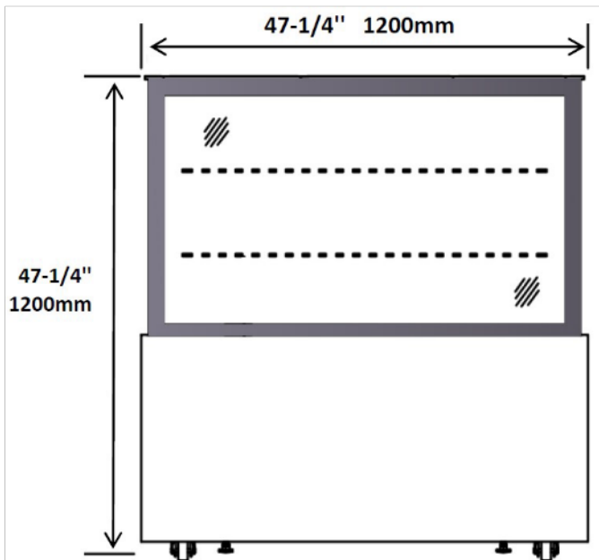
ECD47-2X FRONT
