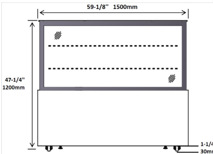
ECD71-2X FRONT
