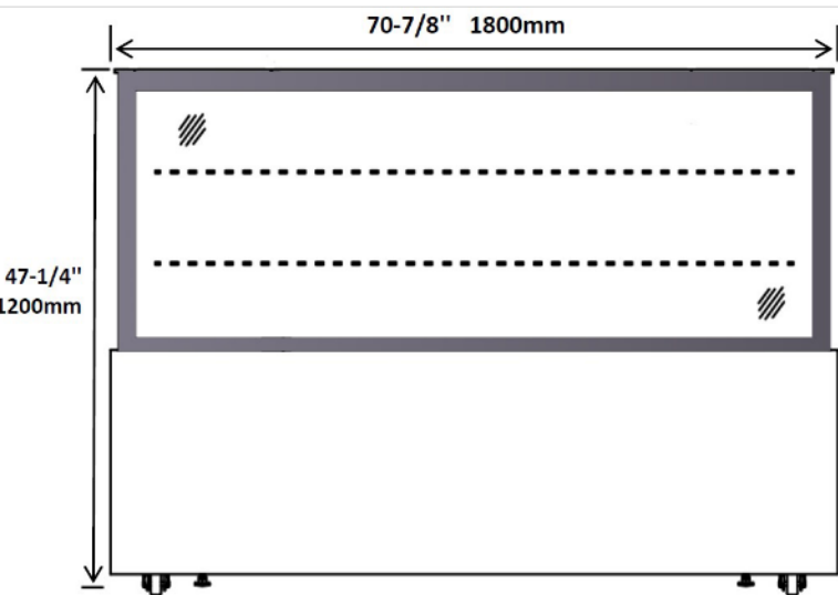
ECD71-2X FRONT
