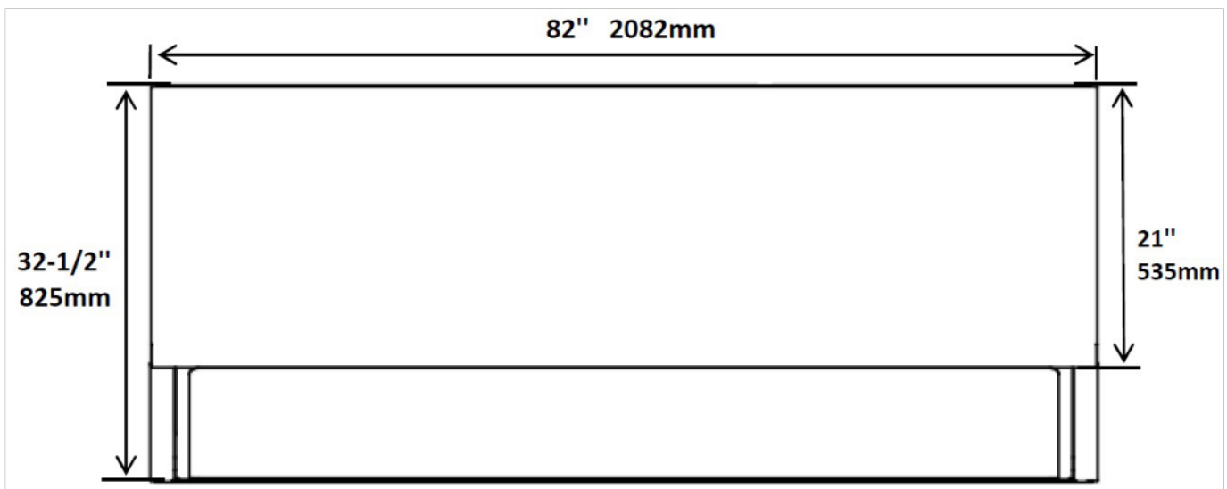
EDC79X TOP VIEW
