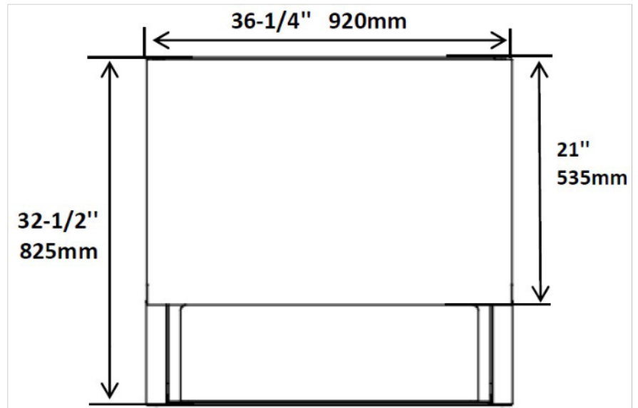
EDC36X TOP VIEW
